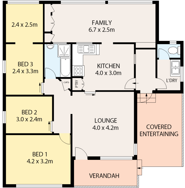
ENTRY LEVEL
